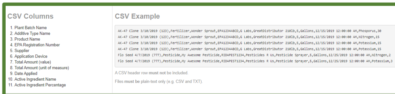
Figure 10: Immature Plant Additive CSV Columns and Example
